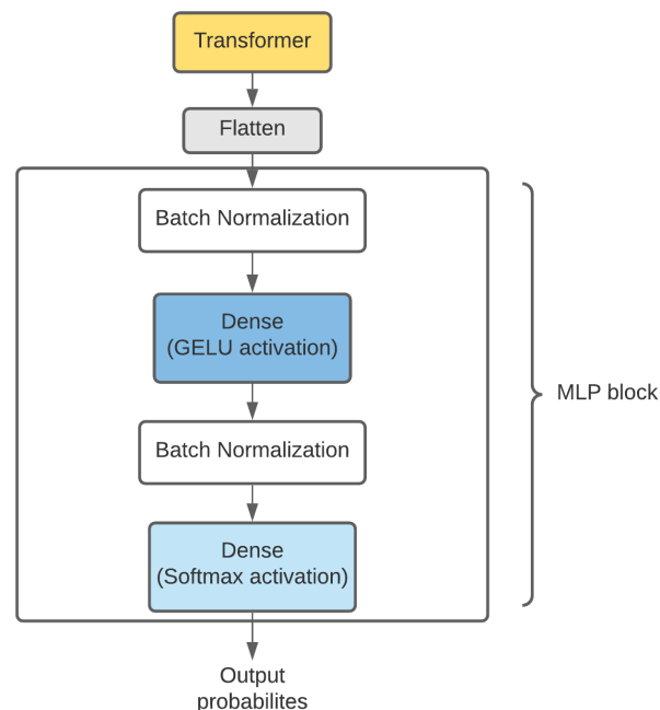
Figure 2. Custom MLP block attached to the Vision Transformer.
