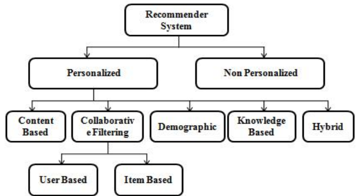
Figure 1. Different types of Recommendation System
