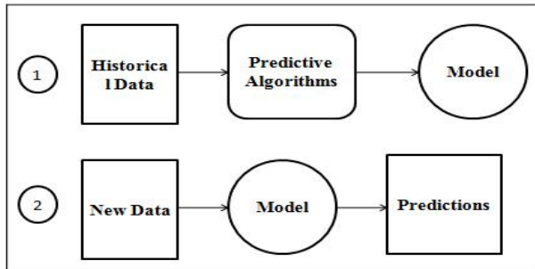
Figure 2. Predictive Analytics
