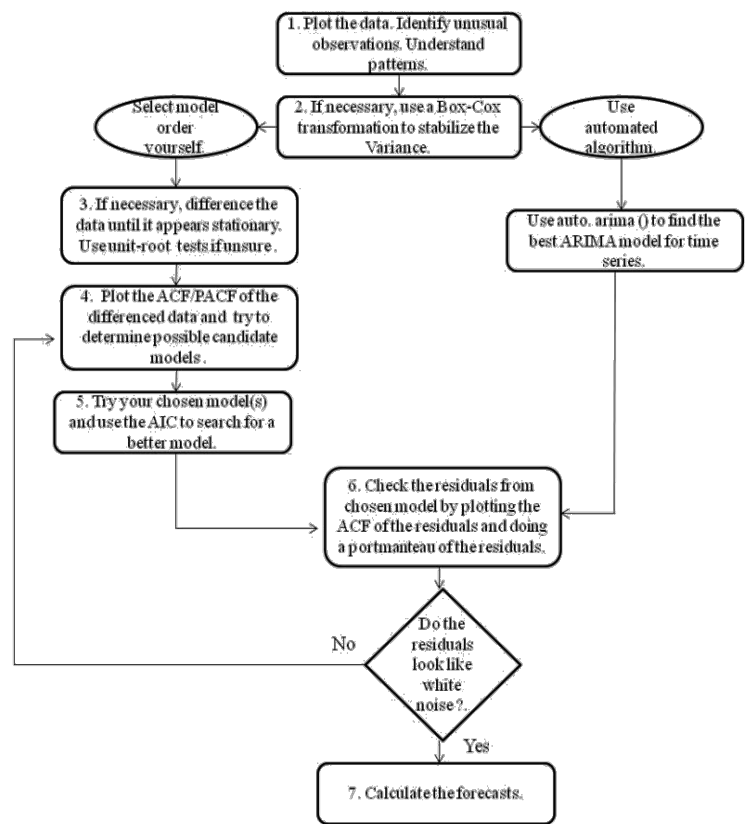
Figure 5. Modelling Procedure for ARIMA
