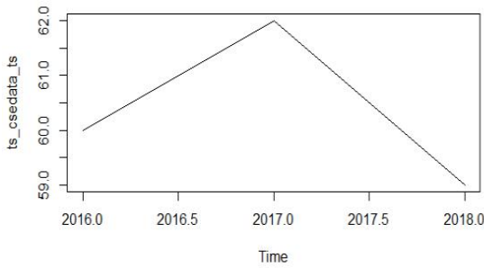
Figure 8. R plot of the input data set
