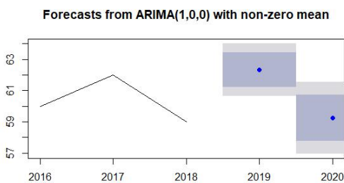
Figure 10. R plot of output from ARIMA forecast
