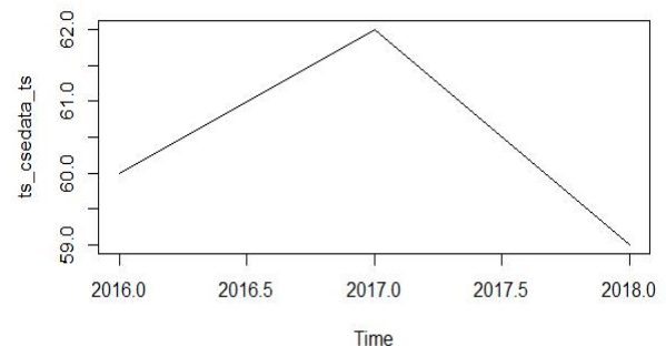
Figure 4. Time series plot of data set
