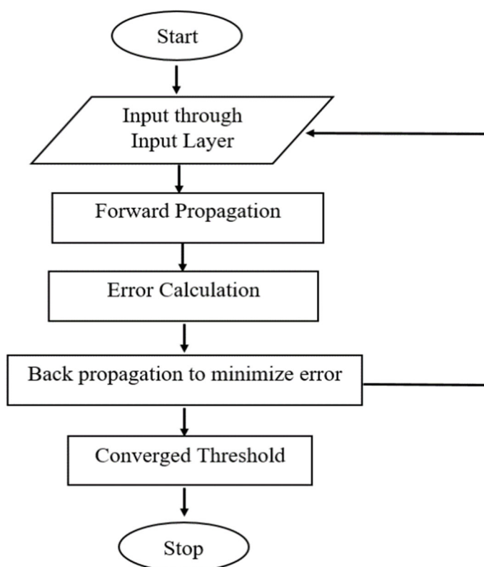
Figure 3. Learning process of the MLP.
