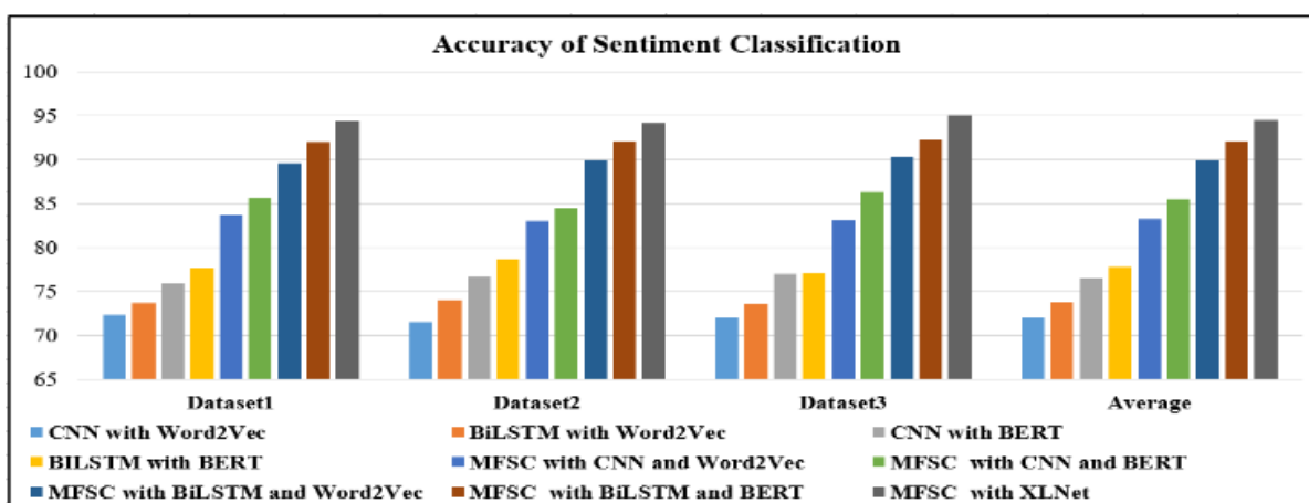
Figure 5. Graphical representation of the performance results with the MFSC model.
