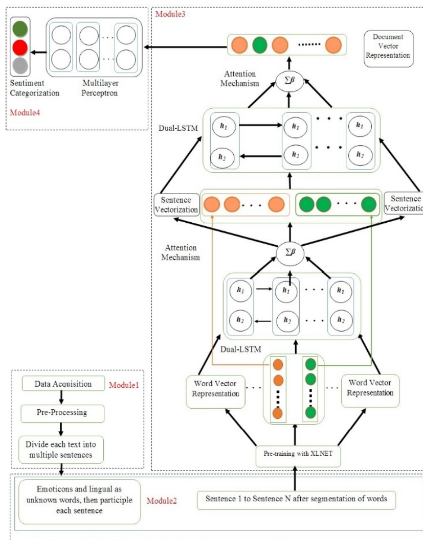
Figure 1. The proposed model.
